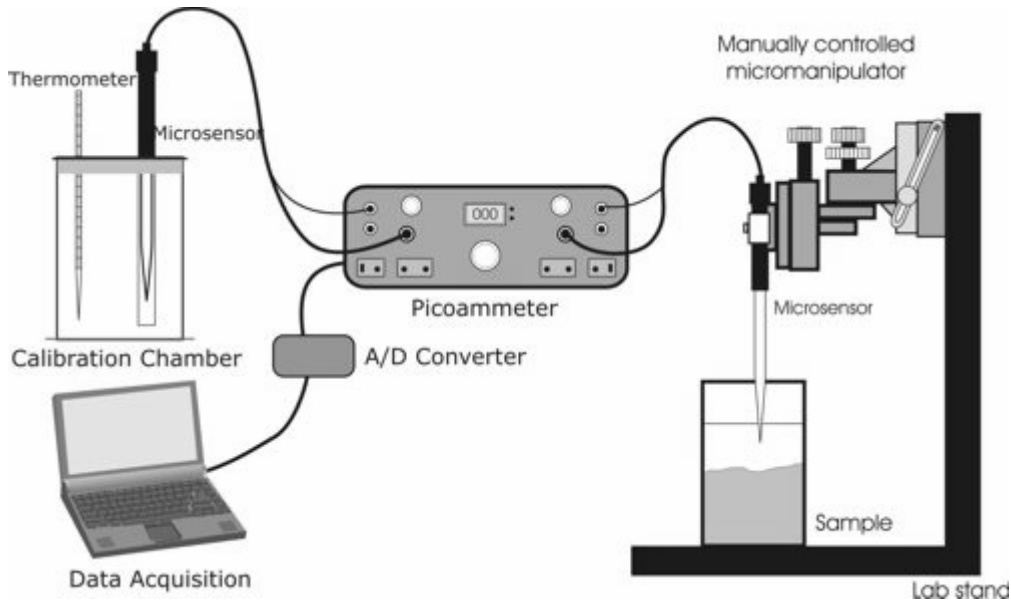
Figure 2. Microelectrode set-up.
