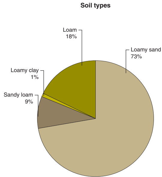
Figure 3: Main soil types in the Rönne Å catchment.
