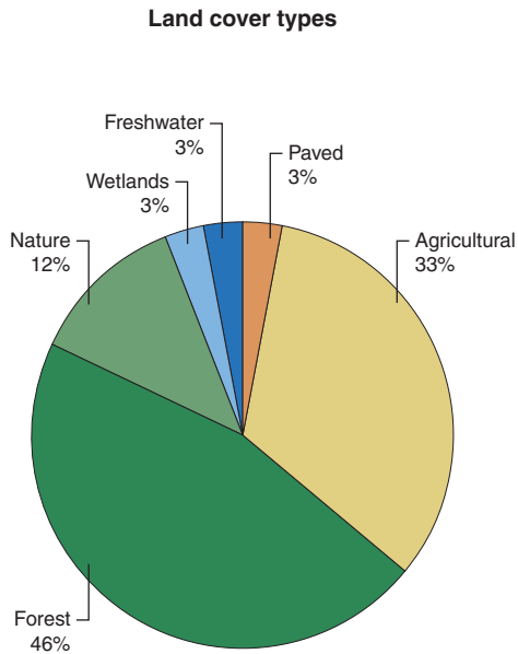
Figure 2: Main land use classes in the Rönne Å catchment.
