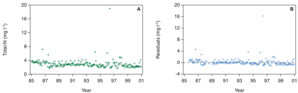
Figure 9: Time series of concentrations of total N and the flow-adjusted concentrations (residuals) during the period 1985-2001. Average concentration of total nitrogen is 2.97 \text{ mg l}^{-1} ( CV=47\% ).
