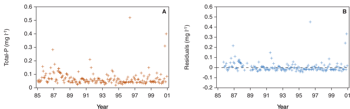
Figure 10: Time-series of flow-adjusted concentrations of total phosphorus and the flow-adjusted concentrations (residuals) during the period 1985-2001. The average concentration of total phosphorus is 0.071 mg l -1 (CV=79%).
