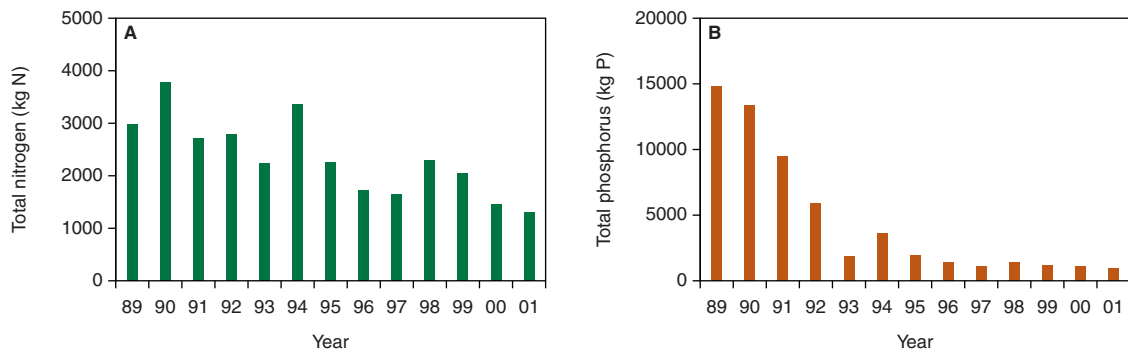
Figure 4: Annual discharge of total nitrogen and total phosphorus from WWTPs in the Rönne Å catchment.
