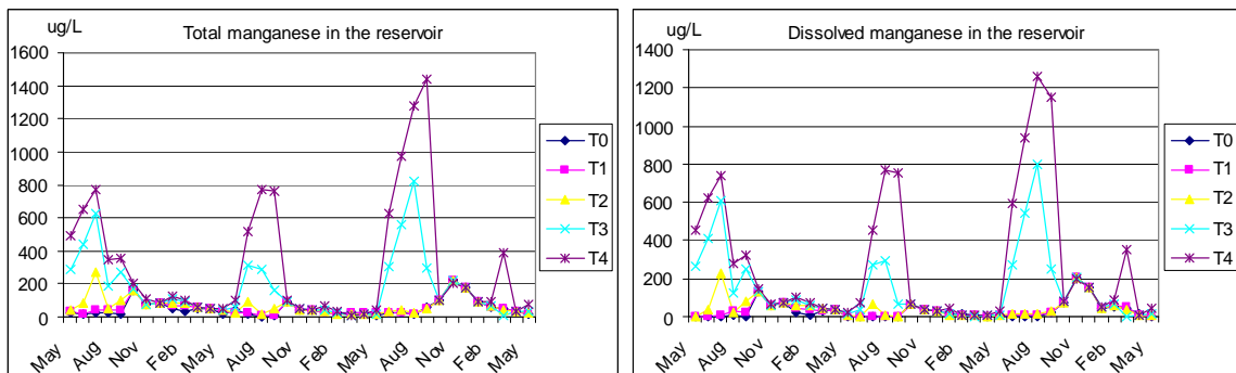
Figure 7. Total and dissolved manganese in the reservoir
