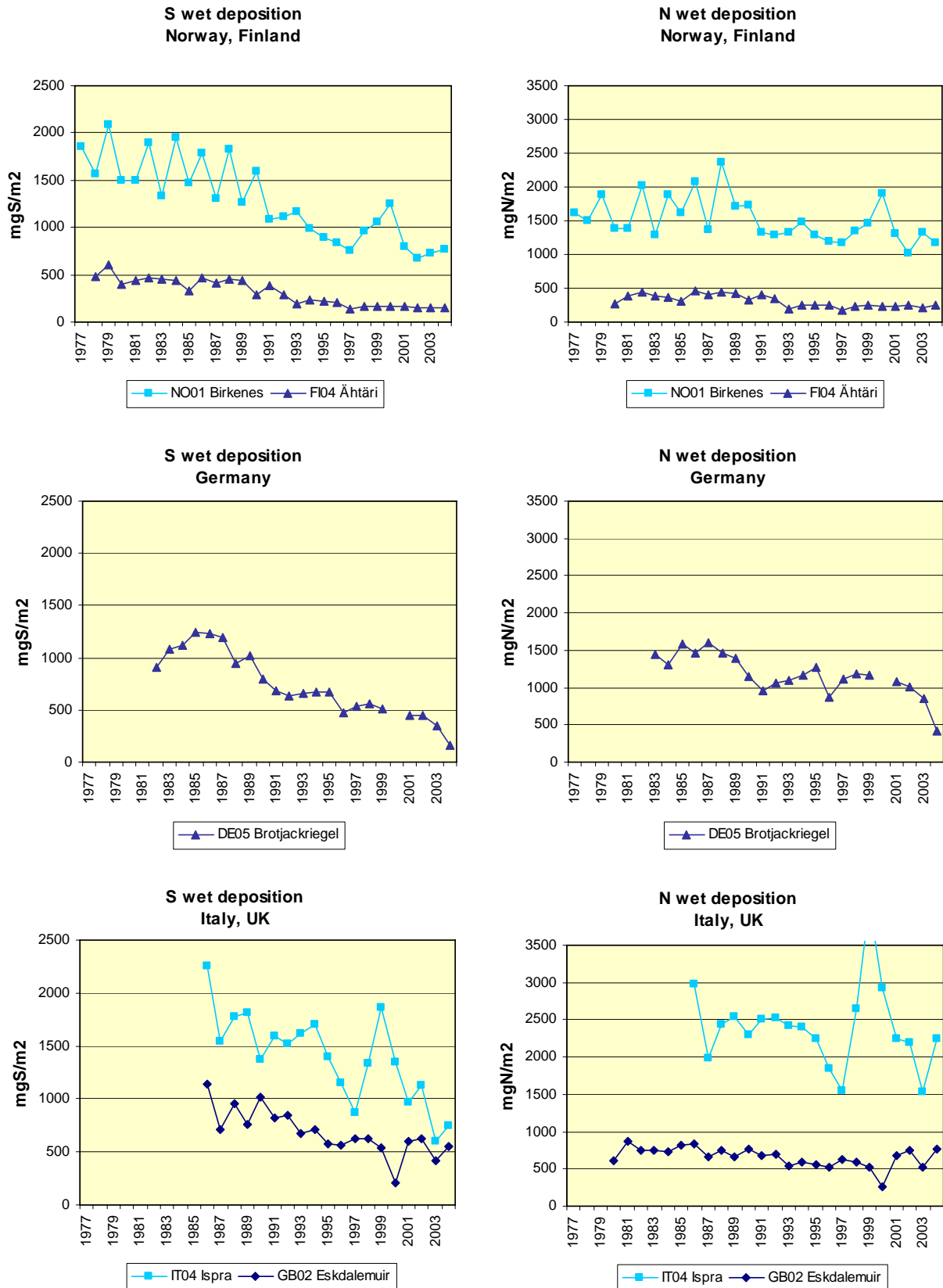
Figure 3. Measured wet deposition of sulphur (left-hand panels) and nitrogen (sum of \text{NH}_4 + \text{NO}_3 ) (right-hand panels) at several EMEP sites in northern, central, western and southern Europe (data from www.emep.int ).
