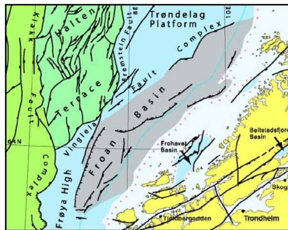
Figure 3. The Foran Basin off Mid-Norway is one possible site for sub-seabed CO 2 storage (NGU, 2004).
