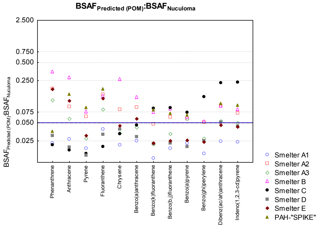
Figure 20. The ratio between the “POM-predicted” biota to sediment accumulation factors (calculated from the POM-SPE-deduced K_{ds} (sediment water partitioning coefficients), K_{ow} s (the octanol:water partitioning coefficients) and the OC-normalized sediment PAH-concentrations) and the actual measured BSAFs for the bivalve Nuculoma tenuis (calculated from the lipid normalized concentrations in the organism and the OC-normalized concentrations in the sediments). The ratio is presented for all sediments and all PAHs (from phenanthrene) presented from left to right with increasing K_{ow} s. The median (0.05) is presented by a blue line. Note logarithmic scale.
