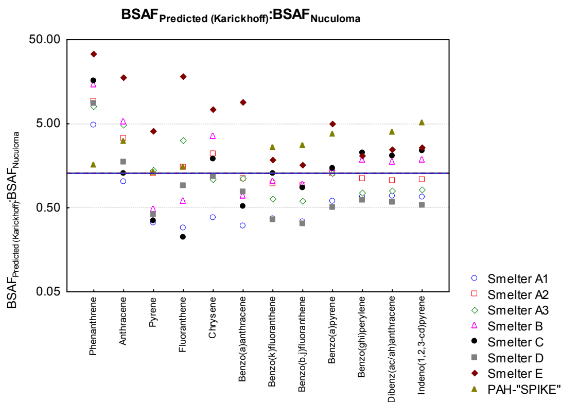
Figure 21. The ratio between the “Karickhoff-predicted” biota to sediment accumulation factors (BSAF=1.62), and the actual measured BSAFs for the bivalve Nuculoma tenuis (calculated from the lipid normalized concentrations in the organism and the OC-normalized concentrations in the sediments). The ratio is presented for all sediments and all PAHs (from phenanthrene) presented from left to right with increasing K_{ow} s. The median (1.49) is presented by a blue line. Note logarithmic scale.
