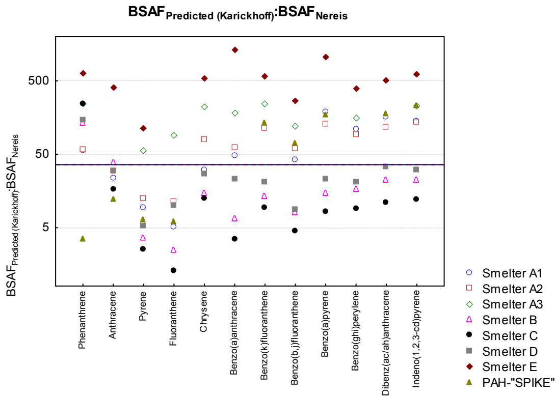
Figure 17. The ratio between the “Karickhoff-predicted” biota to sediment accumulation factors ( BSAF=1.62 ), and the actual measured BSAFs for the polychaete Nereis diversicolor (calculated from the lipid normalized concentrations in the organism and the OC-normalized concentrations in the sediments). The ratio is presented for all sediments and all PAHs (from phenanthrene) presented from left to right with increasing K_{ow} s. The median (36.1) is presented by a blue line. Note logarithmic scale.
