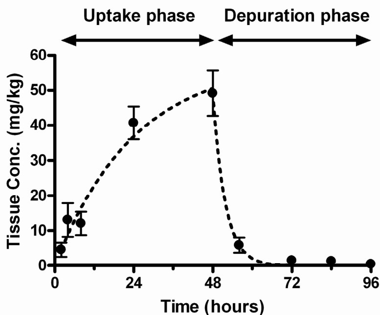
Figure 2. Mean measured ( \pm SD) concentrations of sucralose in fish exposed to 100 mg/L sucralose for 48 hours followed by a 48h depuration phase in clean water.
