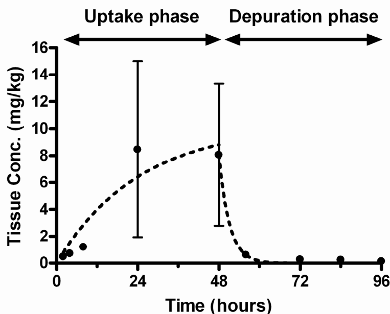
Figure 1. Mean measured ( \pm SD) concentrations of sucralose in fish exposed to 10 mg/L sucralose for 48 hours followed by a 48h depuration phase in clean water.
