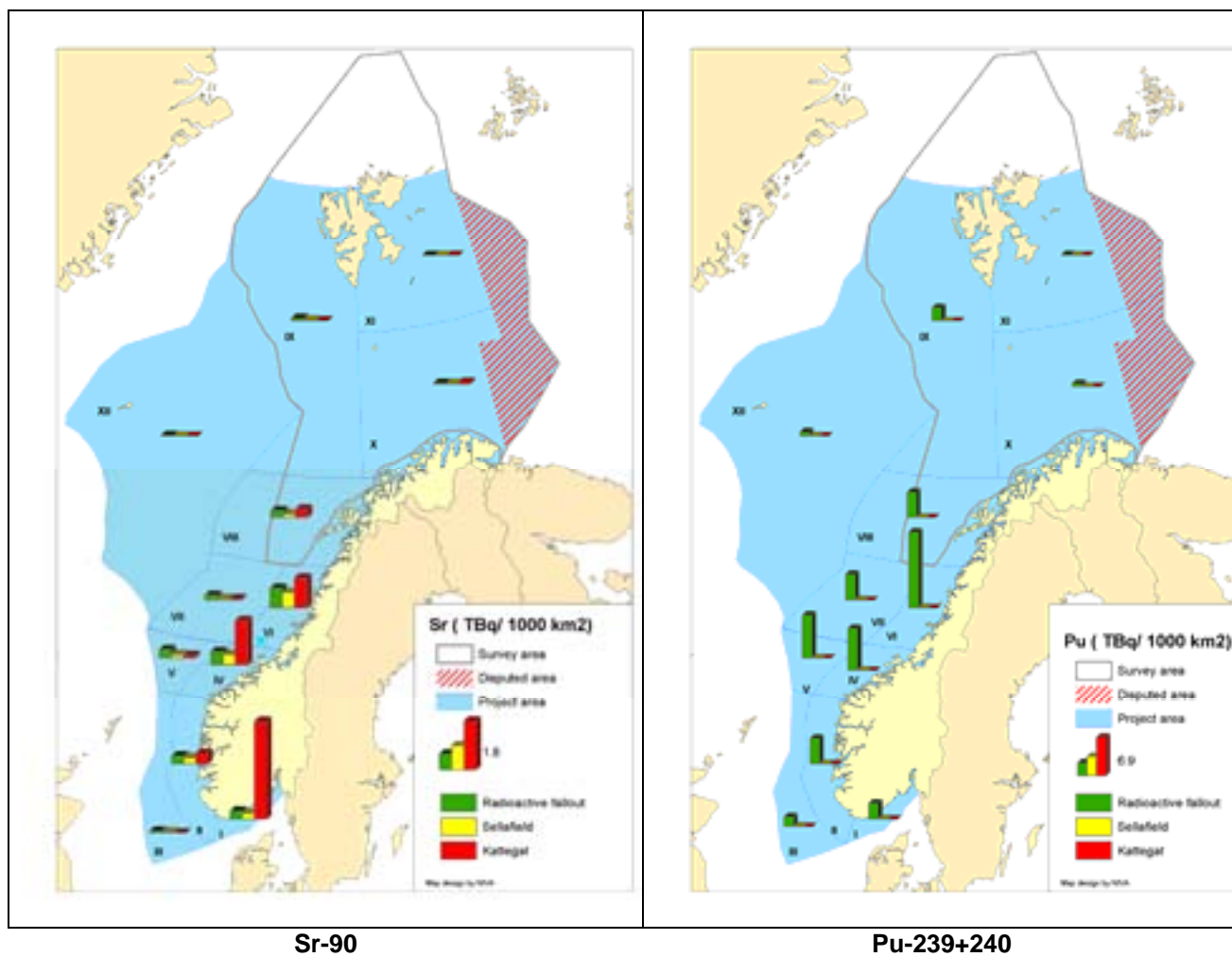
Figure S2. The calculated load of strontium-90 and plutonium-239+240. In this map Kattgat is considered a source for load of radionuclides to Norwegian waters, even though the nuclides originate from discharges to the Baltic.
