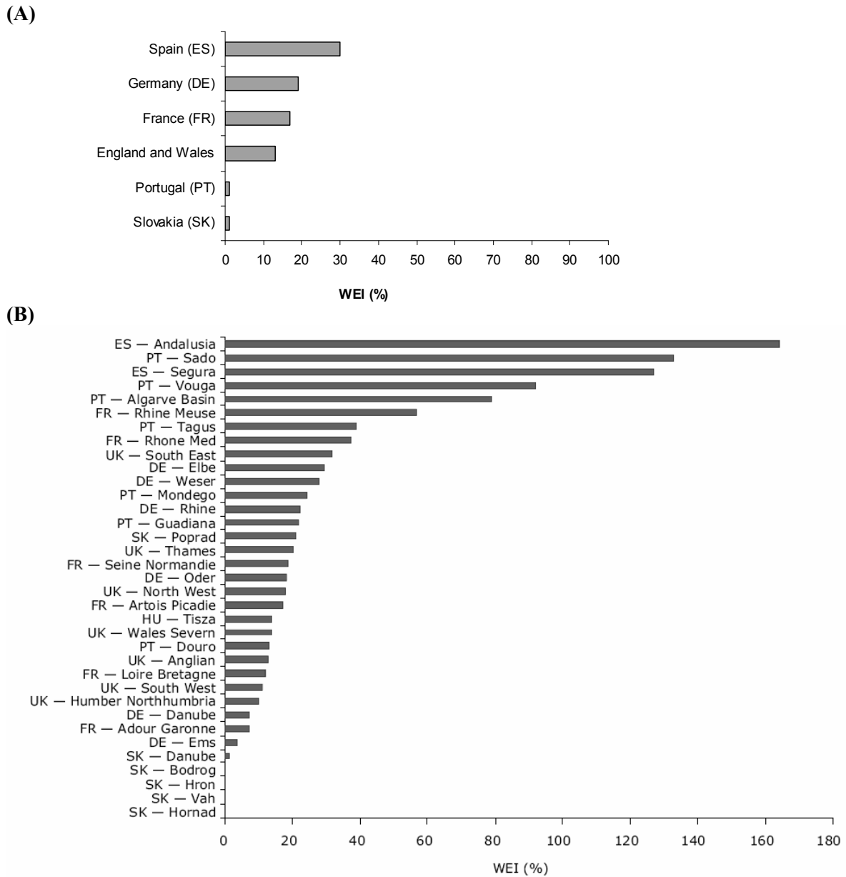
Figure 5. The Water Exploitation Index (WEI) for selected EU countries: results aggregated to national level (A) and to river basin level (B). The WEI is calculated as the ratio of total freshwater abstraction to the total renewable resource. A WEI above 20 % implies that a water resource is under stress and values above 40 % indicate severe water stress and clearly unsustainable use of the water resource. A comparison of the two aggregation levels show e.g. that while Spain appears to have an overall WEI of 30 %, certain Spanish river basins such as Andalusia and Segura have a WEI above 100 %. Source: (A) EEA based on data submitted to the Eurostat, 2007; (B): EEA, 2009.
