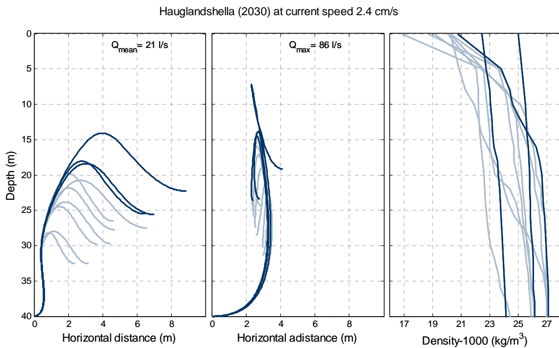
Figure 20. Discharge trapping depth at Hauglandshella calculated for discharge water flows of 21 and 86 l/s in 2030, discharge depth of 40 m, and current speed 2.4 cm/s. Right panel show the different stratification scenarios used. The three situations giving the worst cases are marked with darker colour.
