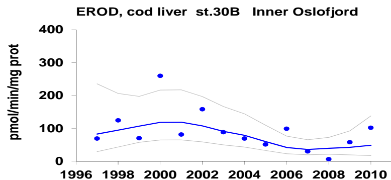
Figure 43. Median activity of cytochrome P4501A (EROD-activity, pmol/min/mg protein) in liver from Atlantic cod collected from southern Norway (cf. Appendix H and see otherwise key to map and detail in Figure 2). There is no limit to classify the results from 2010.
