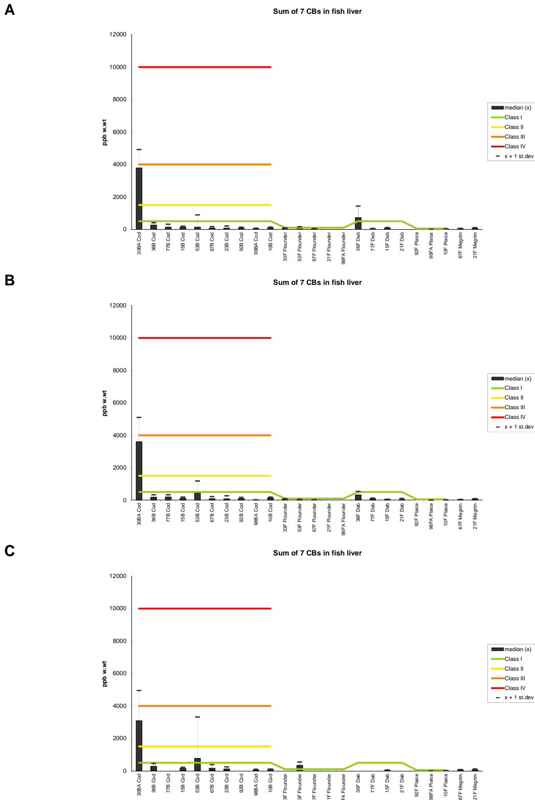
Figure 52. Median, standard deviation and upper limit to Klif Classes or provisional "high background" concentration for sum of 7 PCBs (CB-28, -52, 101, -118, -138, -153 and -180) in fish liver 2008 (A), 2009 (B) and 2010 (C), ppb ( \mu\text{g}/\text{kg} ) wet weight, "Cl. I-B" indicates that only upper limit to Klif Classes or provisional high background concentration is indicated for flatfish, (see maps in Appendix F).
