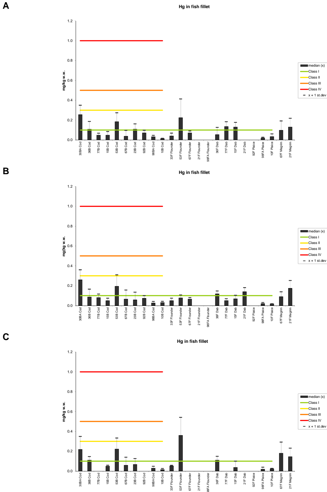
Figure 48. Median, standard deviation and upper limit to Klif Classes or provisional "high background" concentration for mercury in fish fillet 2008 (A), 2009 (B) and 2010 (C), ppm (mg/kg) wet weight, "Cl.-B" indicates that only upper limit to Klif Classes or provisional high background concentration is indicated for flatfish, (see maps in Appendix F).
