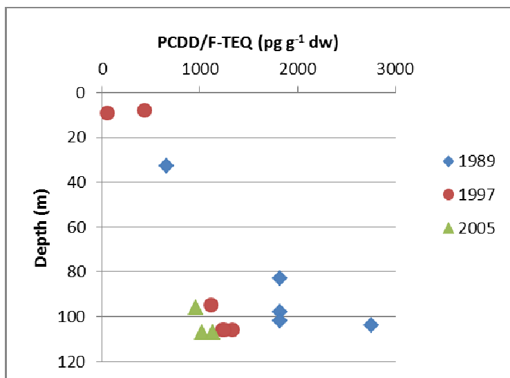
Figure 8. Dioxin analyses in top 0-2cm of sediments in Eidangerfjorden sampled during the period 1989-2005. Norwegian EQS for class V “very bad” is 500 \text{pg g}^{-1} d.w.
