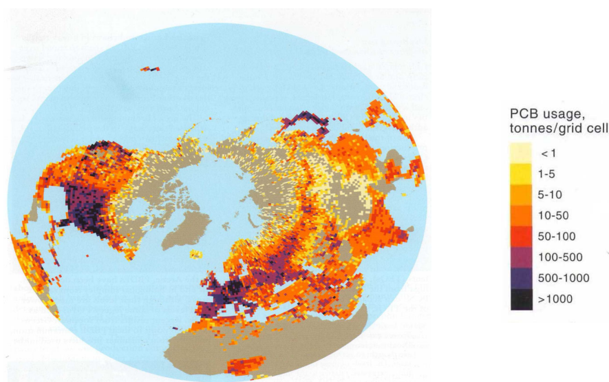
Figure 1. Global PCB usage, tones/grid cell [1]
