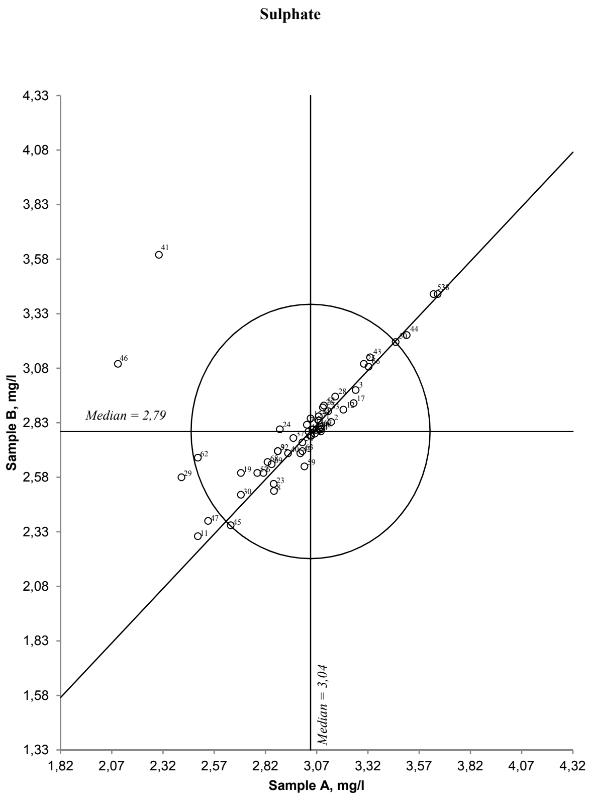
Figure 6. Youdendiagram for sulphate, Samplepair AB Acceptable limit , given by circle, is 20 %
