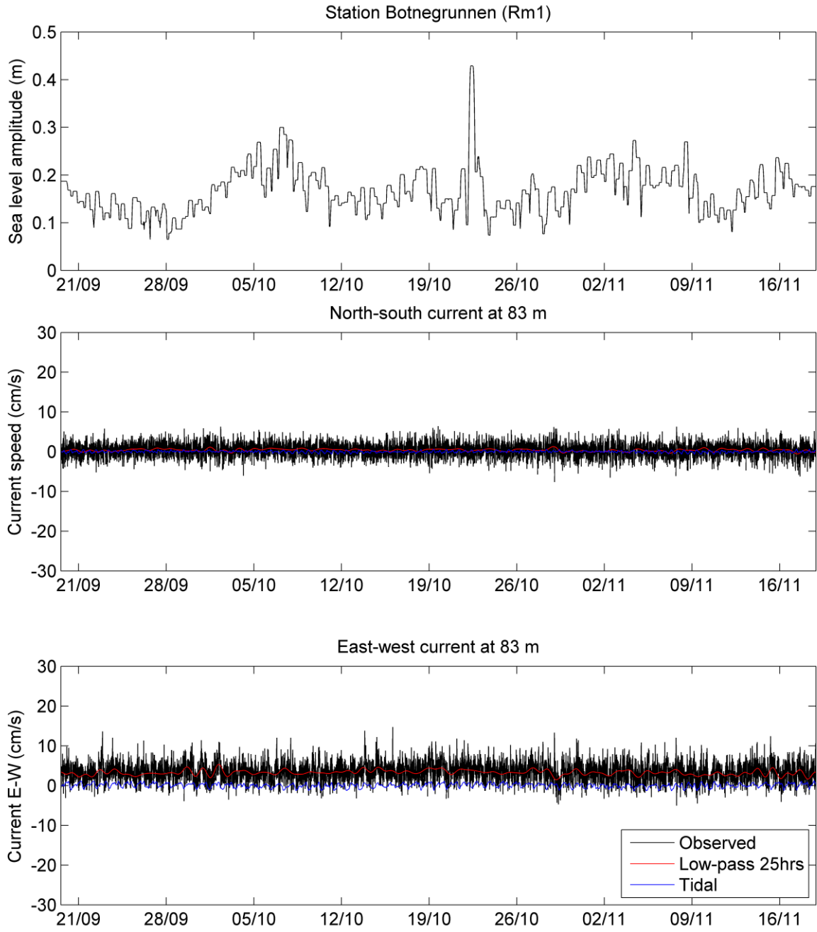
Figure 22. The current 13 m over the bottom at station Botnegrunnen (middle and lower panel) from September to November 2014 plotted as a time series together with the sea level amplitude.
