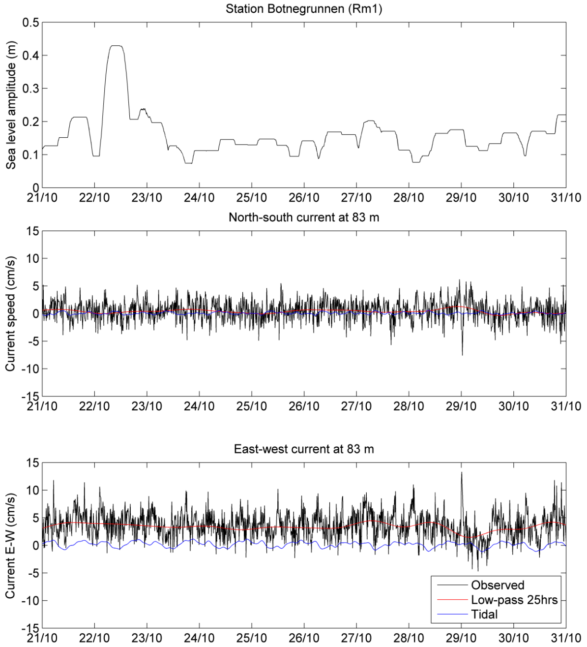
Figure 23. The current 13 m over the bottom at station Botnegruppen (middle and lower panel) plotted as a time series together with the sea level amplitude.
