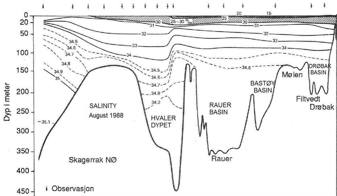
Figure 2. Salinity shown along a transect from the open ocean (Skagerrak) and into the Oslofjord. Surfaces of constant salinity are shown. The thick black line indicates the bathymetry. The figure is taken from Baalsrud and Magnusson (1990).
