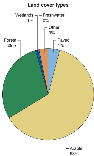
Figure 2: Main land use classes in the Susve catchment.
