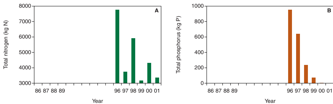
Figure 4: Annual discharge of total nitrogen and total phosphorus from WWTPs in the Susve catchment.
