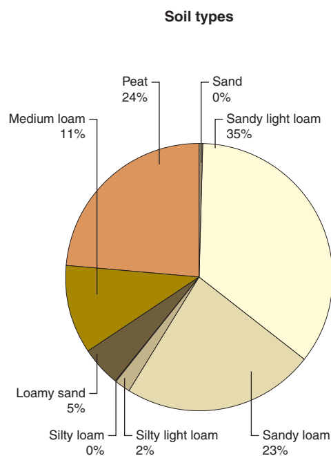
Figure 3: Main soil types in the Susve catchment.
