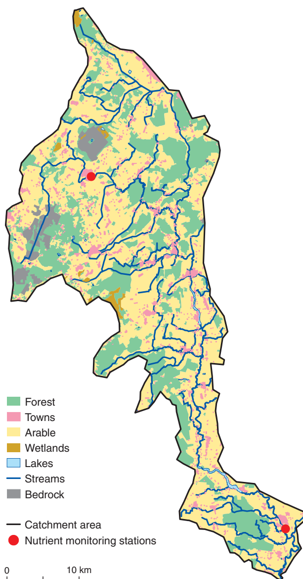
Figure 1: Map showing land use and river network characteristics for the Susve catchment, Lithuania, and existing water quality monitoring stations in the catchment.
