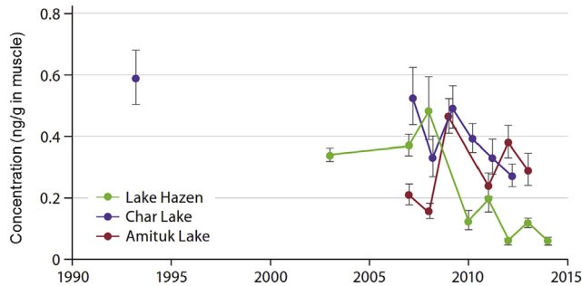
Fig. 28. Trends of C_7 – C_{14} perfluorocarboxylates ( \Sigma PFCAs) in landlocked char muscle from Lake Hazen, Char Lake and Amituk Lake in the Canadian Arctic. (D. Muir, Environment Canada, Burlington, Canada. Unpublished data).
