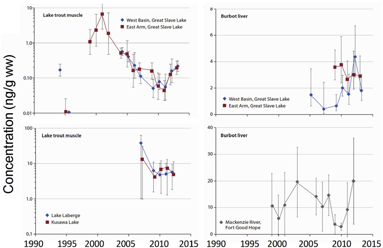
Fig. 29. Trends in C_7 – C_{14} perfluorocarboxylate concentration in lake trout muscle and burbot liver from Great Slave Lake (GSL) (Muir et al. [99]; Evans and Muir, unpubl. data), lake trout muscle from Lake Laberge and Kusawa Lake (Stern et al. [100]), and burbot liver from Fort Good Hope, Mackenzie River [102].
