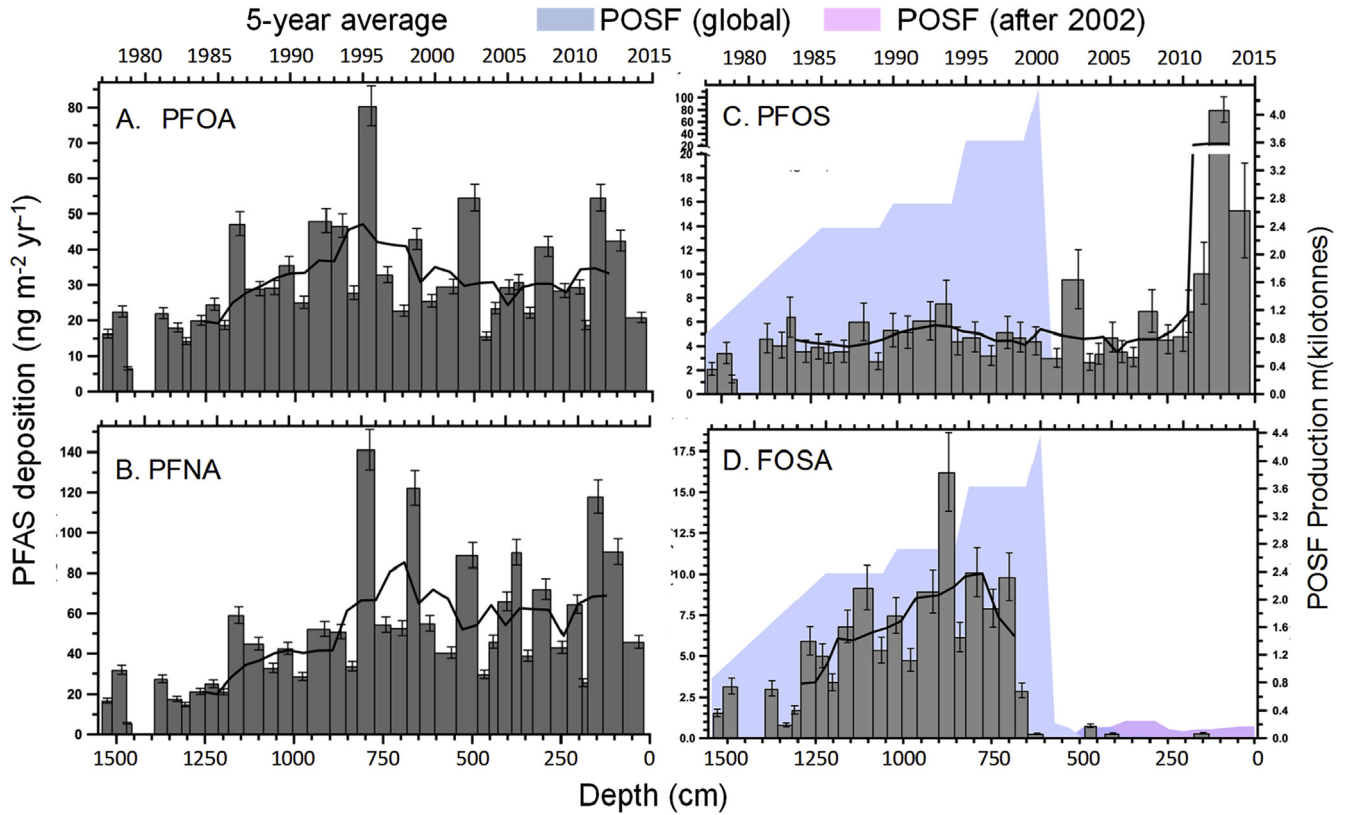
Fig. 26. Estimated annual deposition fluxes ( \text{ng}/(\text{m}^2 \cdot \text{yr}) ) on the Devon Ice Cap: (A) PFOA, (b) PFNA, (C) PFOS and (D) FOSA, with global POSF production from 1977 to 2003 and POSF production for Western Europe, Japan, United States and China from 2003 to 2015 [27,157]. Solid black lines represent 5-year moving averages. Redrawn from Pickard et al. [95].
