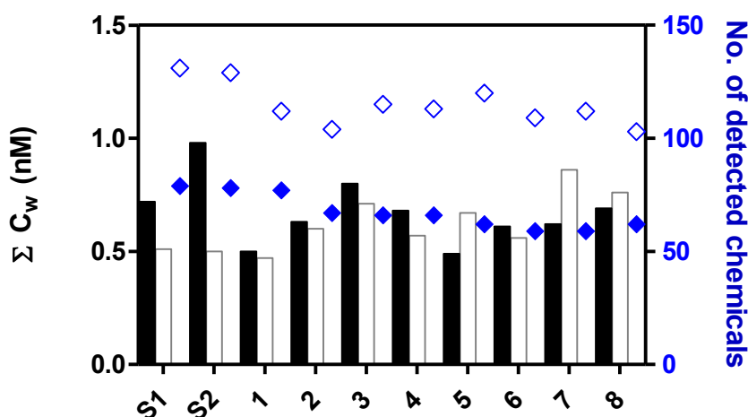
315 Fig. 2 The sum of freely dissolved molar concentrations of chemicals in water ( C_w ), estimated from 316 their amounts analyzed in passive samplers (bar graph) and a number of chemicals detected 317 in the samples (diamond); SR samples (black bar and blue diamond) and ED samples (white 318 bar and empty diamond). S1-2 samples from stationary exposure of samplers downstream of 319 Bratislava (Slovakia); 1-8 samples from a mobile sampling of river stretches.
