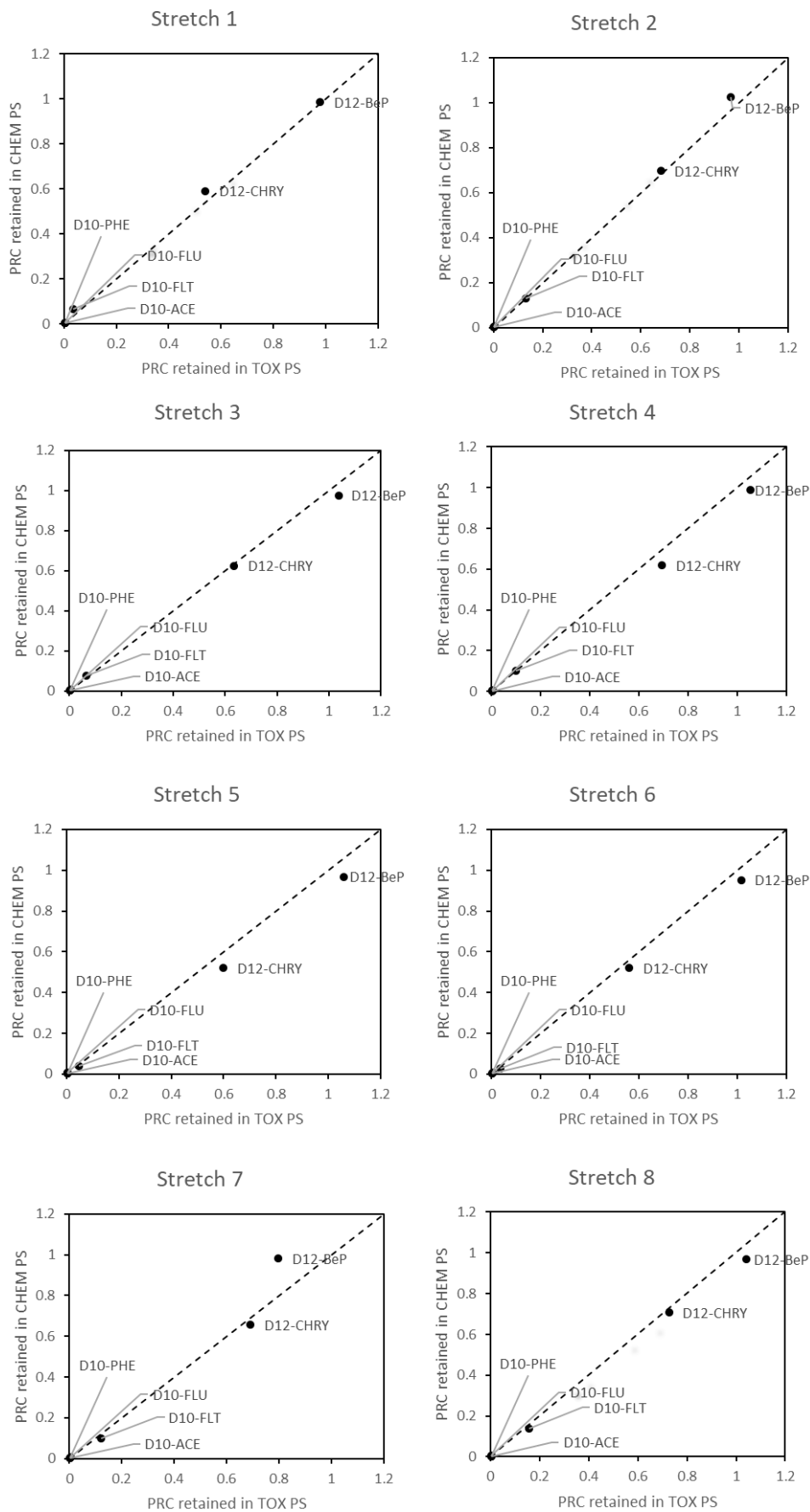
Fig. S2 Comparison of PRC fractions retained in LDPE sheets in two co-deployed DPS devices (TOX PS and CHEM PS) in parallel in 8 Danube stretches
