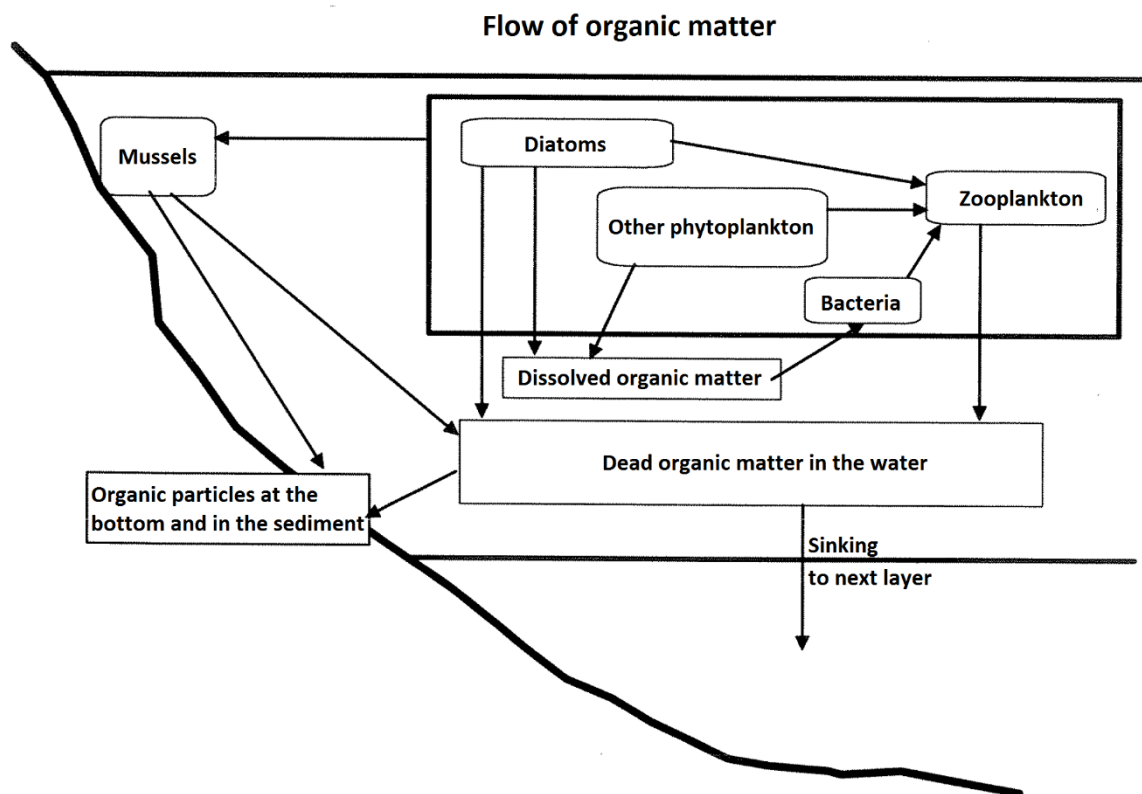
Figur 44. Schematic illustration of the flow of organic matter within one layer of the NIVA Fjord model. In addition to the processes described in the figure, organic matter can be introduced as point sources in each layer and exchanged horizontally with connected basins.
