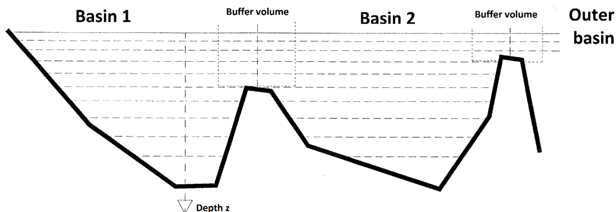
Figur 46. Schematic illustration of the division of the water masses of a fjord system into basins and vertical layers.
