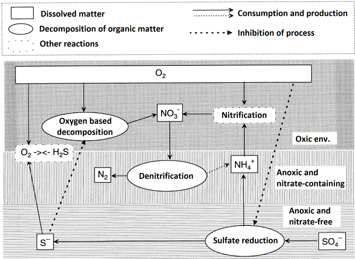
Figur 45. Schematic illustration of the processes included in the NIVA Fjord model to represent decomposition of organic matter and oxygen consumption.
