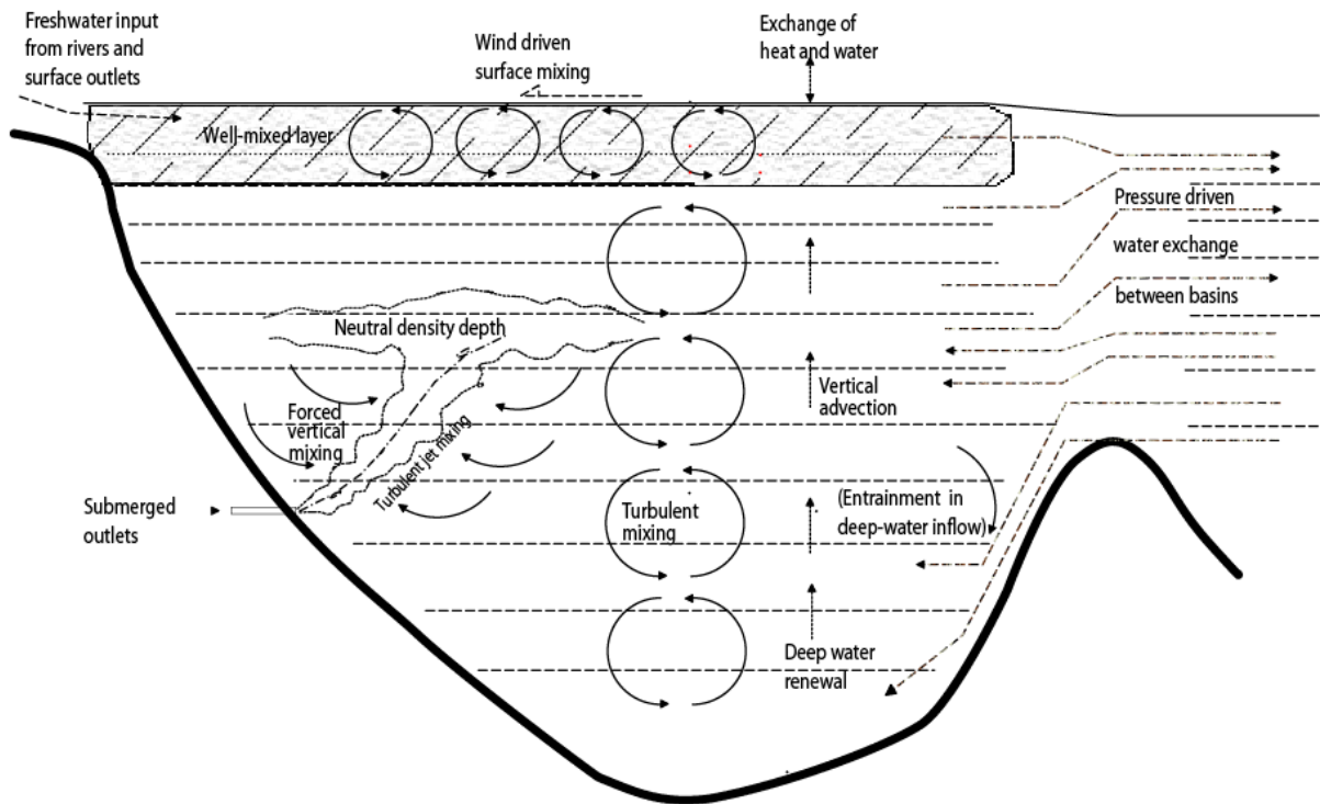
Figur 47. Illustration of the different physical exchange processes that are included in the NIVA Fjord model.
